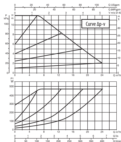
EVOPLUS B 120/250.40 SAN M
